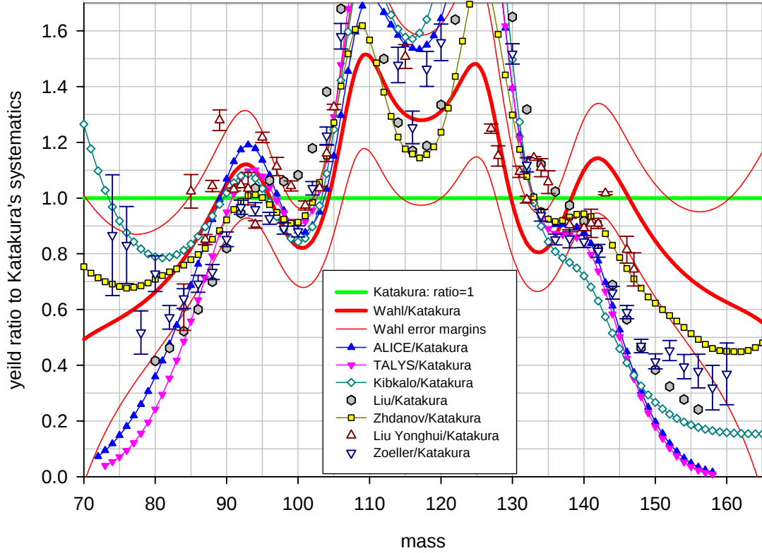
Benchmark A: ^{238}\text{U} at 20-22 MeV, post neutron emission yield ratios to Katakura's systematics lower graph: partial plot (very low and high values omitted).
